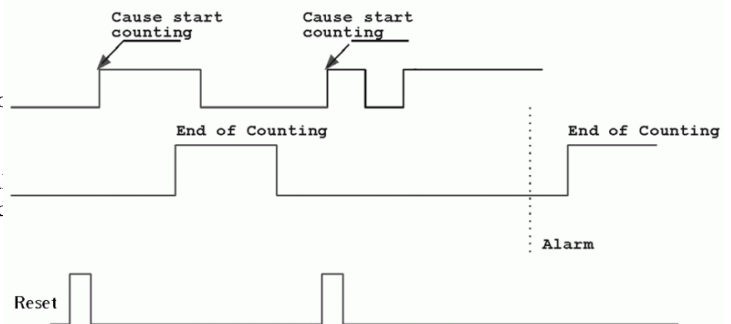
Response Time Monitor Waveform
